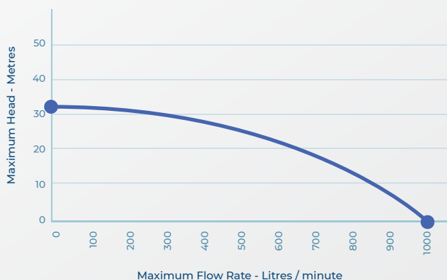
MH30-2 PUMP PERFORMANCE CURVE
