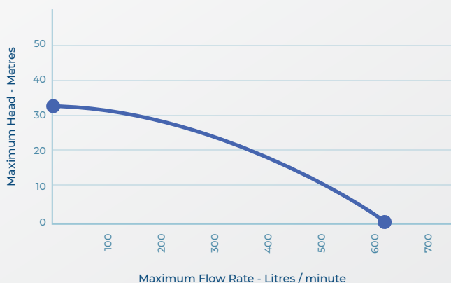
MH20-2 PUMP PERFORMANCE CURVE
