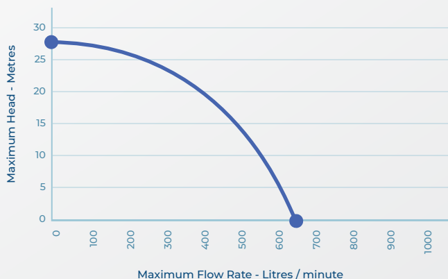
MYD20E PUMP PERFORMANCE CURVE
