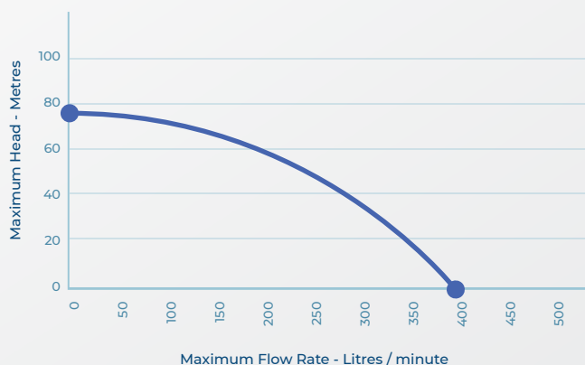
MH15-SHP PUMP PERFORMANCE CURVE
